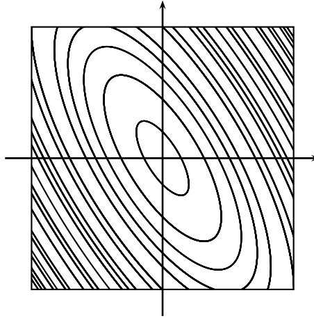
FIGURE 1. a = -1, b = -1, c = 2
